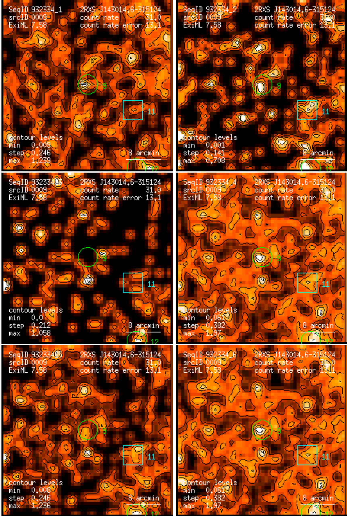
Figure 9: RASS 932334: detection 0009: band rate images, Gaussian filter: (1) PSPC channels 11 – 41, (2) 52 – 90, (3) 91 – 201, (4) 11 – 235, (5) 52 – 201, (6) 11 – 201. Broad band rates in counts/ks. Band rate contour levels in counts/ks/arcmin 2 .
