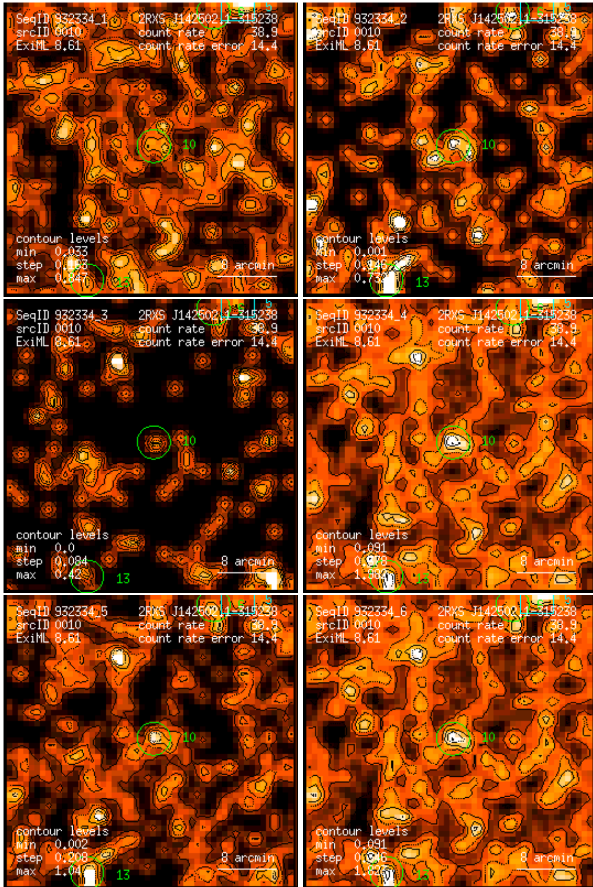
Figure 10: RASS 932334: detection 0010: band rate images, Gaussian filter: (1) PSPC channels 11 – 41, (2) 52 – 90, (3) 91 – 201, (4) 11 – 235, (5) 52 – 201, (6) 11 – 201. Broad band rates in counts/ks. Band rate contour levels in counts/ks/arcmin 2 .
