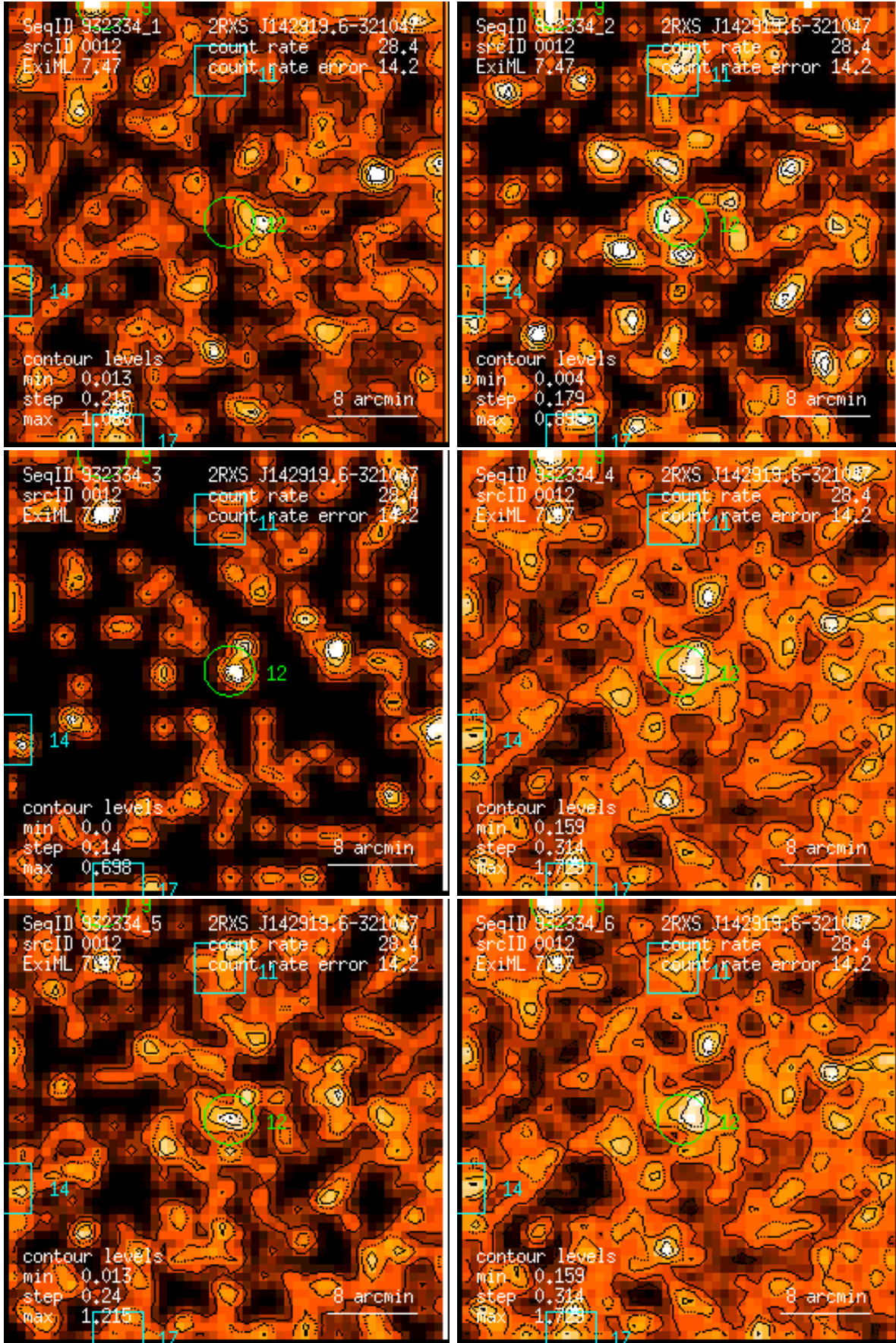
Figure 12: RASS 932334: detection 0012: band rate images, Gaussian filter: (1) PSPC channels 11 – 41, (2) 52 – 90, (3) 91 – 201, (4) 11 – 235, (5) 52 – 201, (6) 11 – 201. Broad band rates in counts/ks. Band rate contour levels in counts/ks/arcmin 2 .
