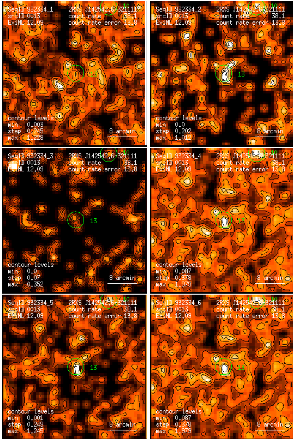
Figure 13: RASS 932334: detection 0013: band rate images, Gaussian filter: (1) PSPC channels 11 – 41, (2) 52 – 90, (3) 91 – 201, (4) 11 – 235, (5) 52 – 201, (6) 11 – 201. Broad band rates in counts/ks. Band rate contour levels in counts/ks/arcmin 2 .
