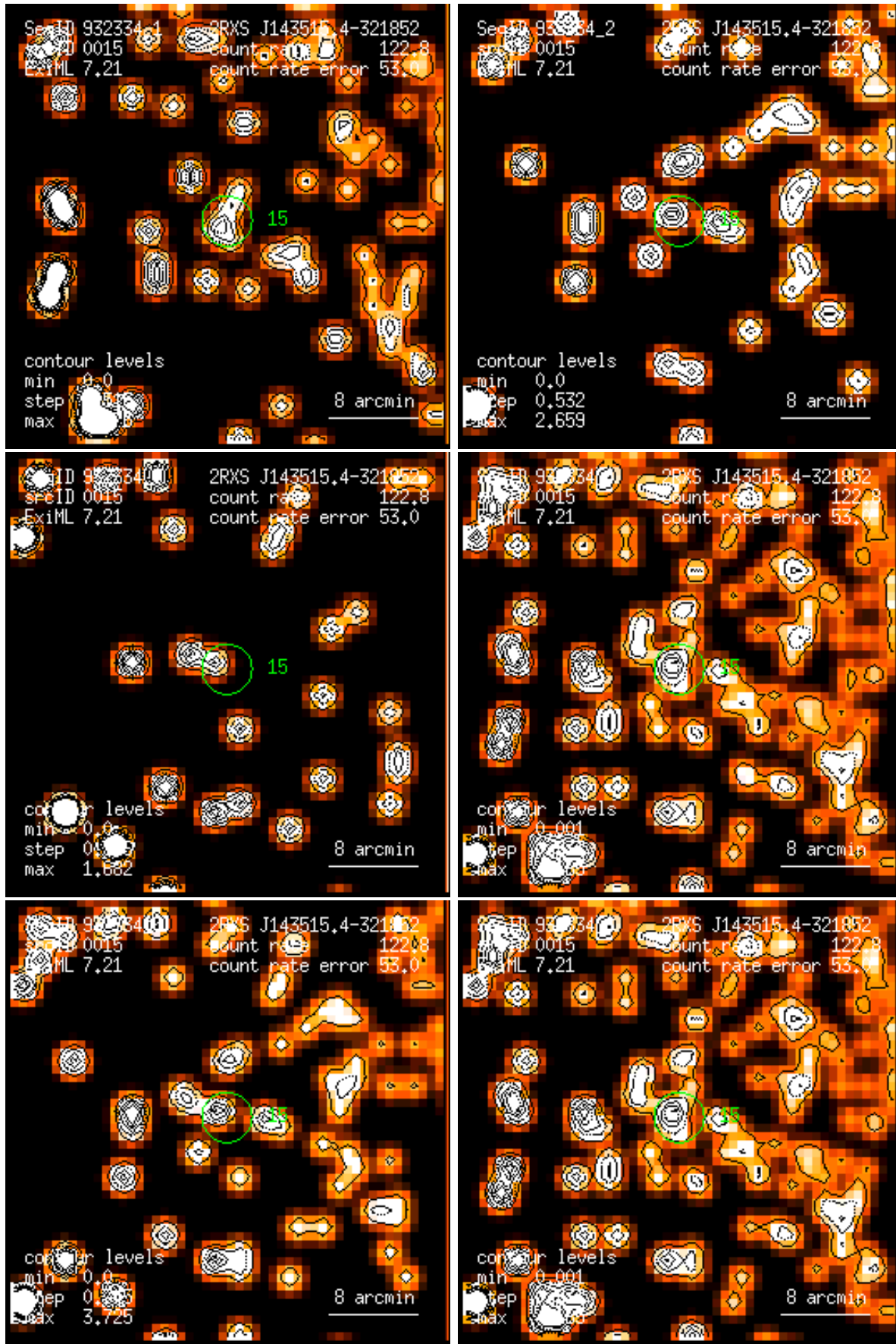
Figure 15: RASS 932334: detection 0015: band rate images, Gaussian filter: (1) PSPC channels 11 – 41, (2) 52 – 90, (3) 91 – 201, (4) 11 – 235, (5) 52 – 201, (6) 11 – 201. Broad band rates in counts/ks. Band rate contour levels in counts/ks/arcmin 2 .
