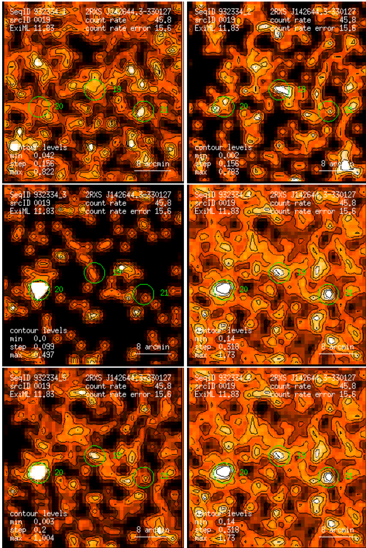
Figure 19: RASS 932334: detection 0019: band rate images, Gaussian filter: (1) PSPC channels 11 – 41, (2) 52 – 90, (3) 91 – 201, (4) 11 – 235, (5) 52 – 201, (6) 11 – 201. Broad band rates in counts/ks. Band rate contour levels in counts/ks/arcmin 2 .
