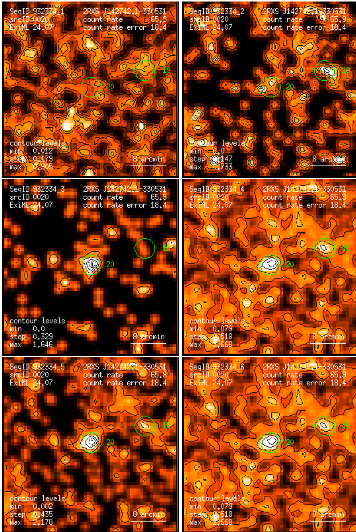
Figure 20: RASS 932334: detection 0020: band rate images, Gaussian filter: (1) PSPC channels 11 – 41, (2) 52 – 90, (3) 91 – 201, (4) 11 – 235, (5) 52 – 201, (6) 11 – 201. Broad band rates in counts/ks. Band rate contour levels in counts/ks/arcmin 2 .
