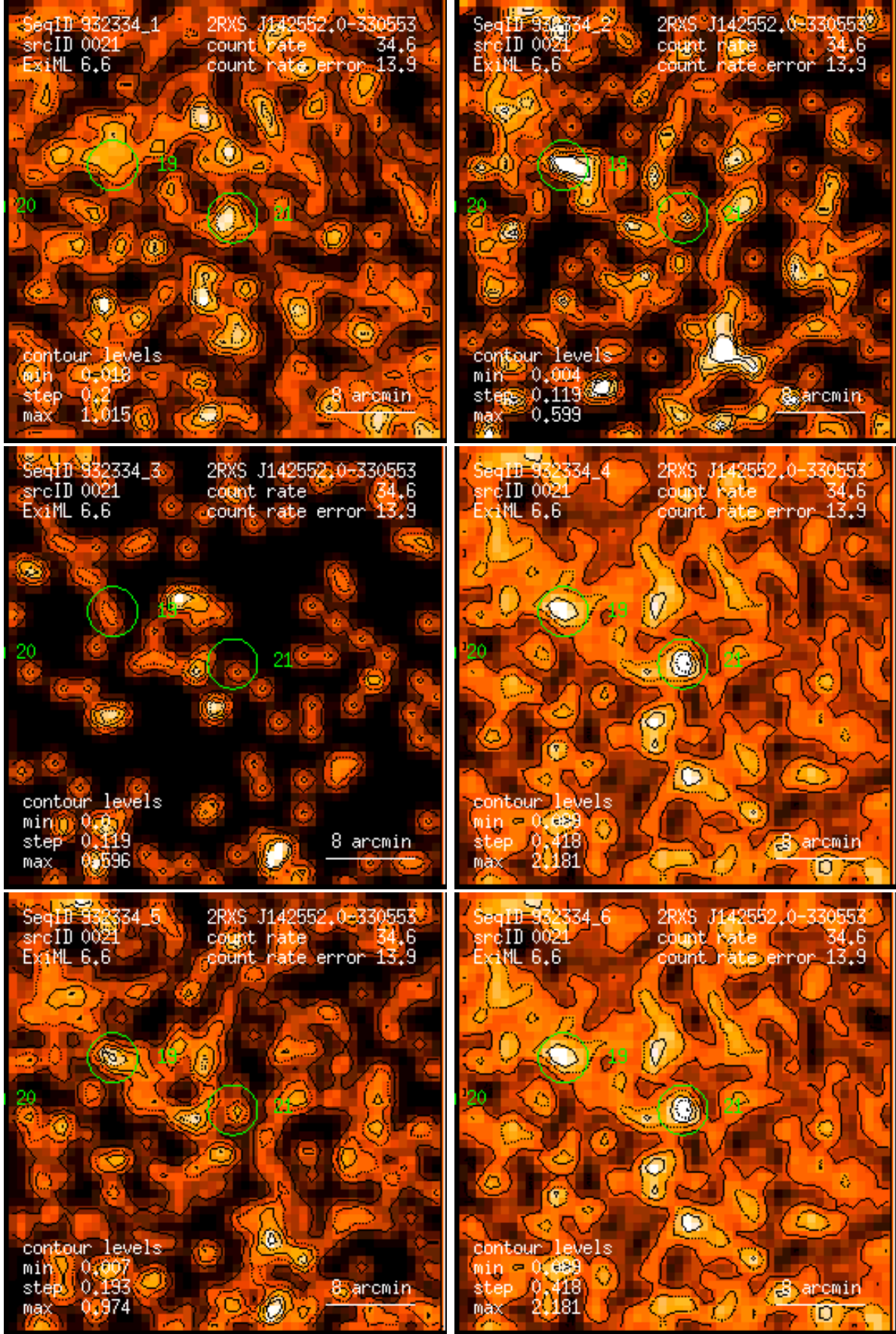
Figure 21: RASS 932334: detection 0021: band rate images, Gaussian filter: (1) PSPC channels 11 – 41, (2) 52 – 90, (3) 91 – 201, (4) 11 – 235, (5) 52 – 201, (6) 11 – 201. Broad band rates in counts/ks. Band rate contour levels in counts/ks/arcmin 2 .
