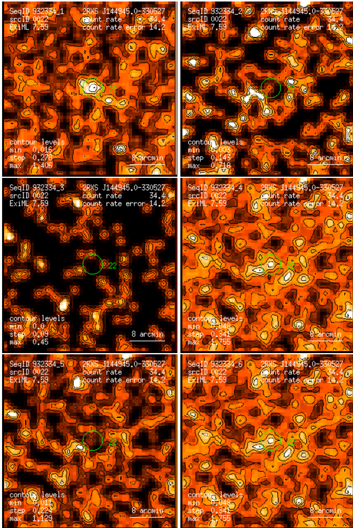
Figure 22: RASS 932334: detection 0022: band rate images, Gaussian filter: (1) PSPC channels 11 – 41, (2) 52 – 90, (3) 91 – 201, (4) 11 – 235, (5) 52 – 201, (6) 11 – 201. Broad band rates in counts/ks. Band rate contour levels in counts/ks/arcmin 2 .
