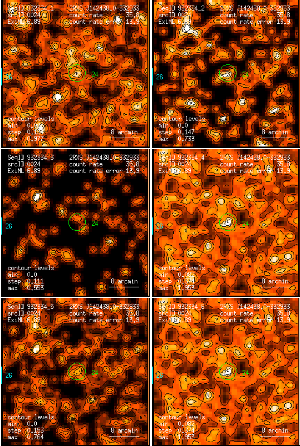
Figure 24: RASS 932334: detection 0024: band rate images, Gaussian filter: (1) PSPC channels 11 – 41, (2) 52 – 90, (3) 91 – 201, (4) 11 – 235, (5) 52 – 201, (6) 11 – 201. Broad band rates in counts/ks. Band rate contour levels in counts/ks/arcmin 2 .
