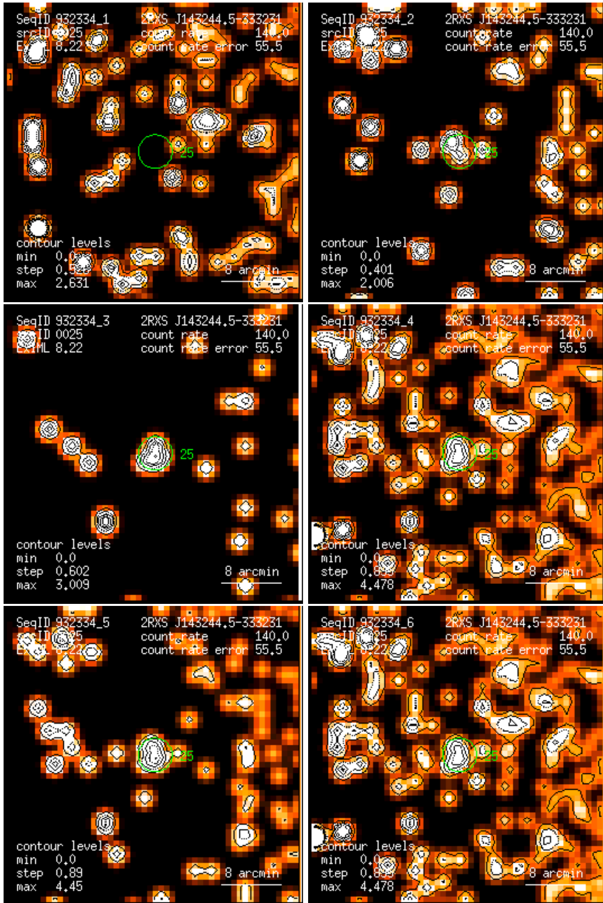
Figure 25: RASS 932334: detection 0025: band rate images, Gaussian filter: (1) PSPC channels 11 – 41, (2) 52 – 90, (3) 91 – 201, (4) 11 – 235, (5) 52 – 201, (6) 11 – 201. Broad band rates in counts/ks. Band rate contour levels in counts/ks/arcmin 2 .
