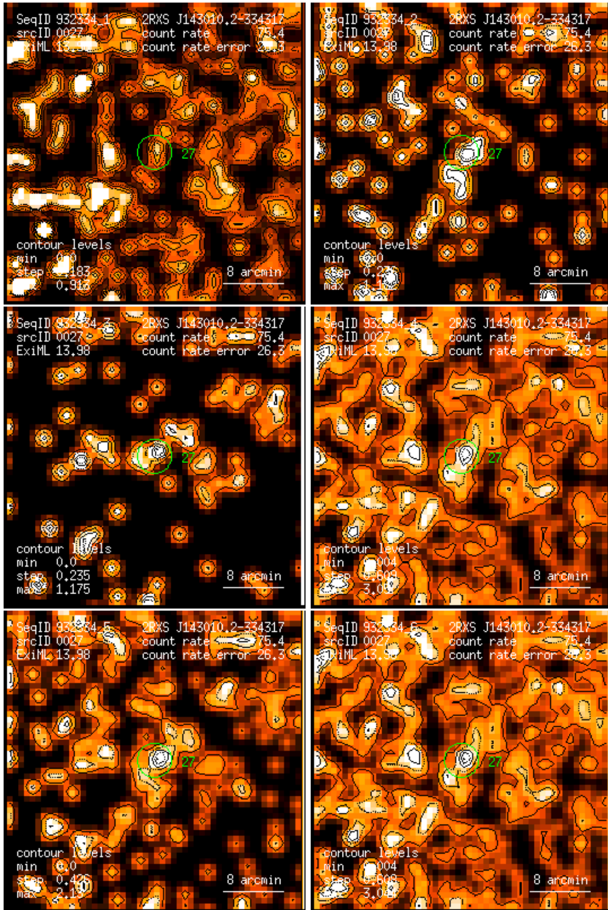
Figure 27: RASS 932334: detection 0027: band rate images, Gaussian filter: (1) PSPC channels 11 – 41, (2) 52 – 90, (3) 91 – 201, (4) 11 – 235, (5) 52 – 201, (6) 11 – 201. Broad band rates in counts/ks. Band rate contour levels in counts/ks/arcmin 2 .
