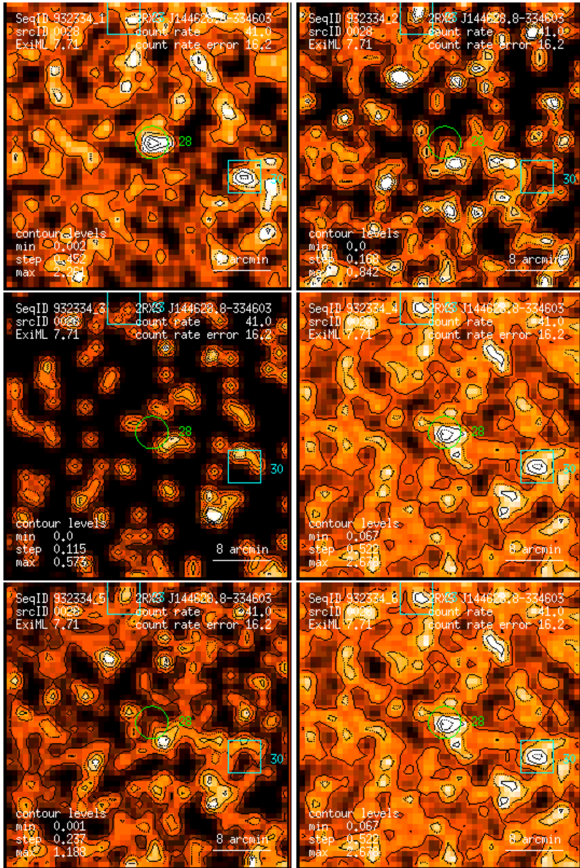
Figure 28: RASS 932334: detection 0028: band rate images, Gaussian filter: (1) PSPC channels 11 – 41, (2) 52 – 90, (3) 91 – 201, (4) 11 – 235, (5) 52 – 201, (6) 11 – 201. Broad band rates in counts/ks. Band rate contour levels in counts/ks/arcmin 2 .
