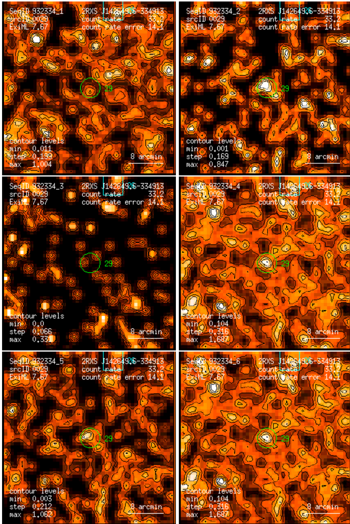
Figure 29: RASS 932334: detection 0029: band rate images, Gaussian filter: (1) PSPC channels 11 – 41, (2) 52 – 90, (3) 91 – 201, (4) 11 – 235, (5) 52 – 201, (6) 11 – 201. Broad band rates in counts/ks. Band rate contour levels in counts/ks/arcmin 2 .
