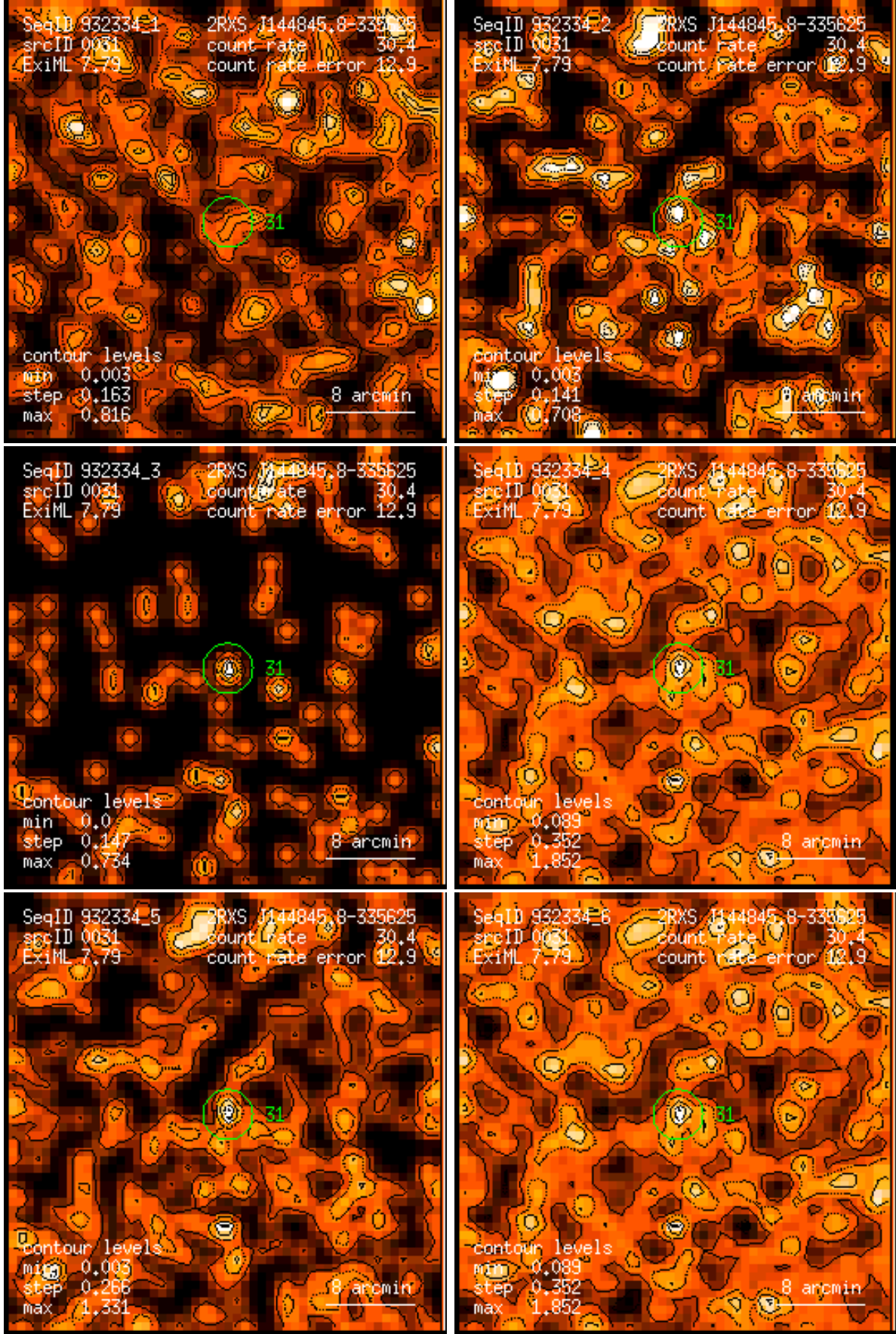
Figure 31: RASS 932334: detection 0031: band rate images, Gaussian filter: (1) PSPC channels 11 – 41, (2) 52 – 90, (3) 91 – 201, (4) 11 – 235, (5) 52 – 201, (6) 11 – 201. Broad band rates in counts/ks. Band rate contour levels in counts/ks/arcmin 2 .
