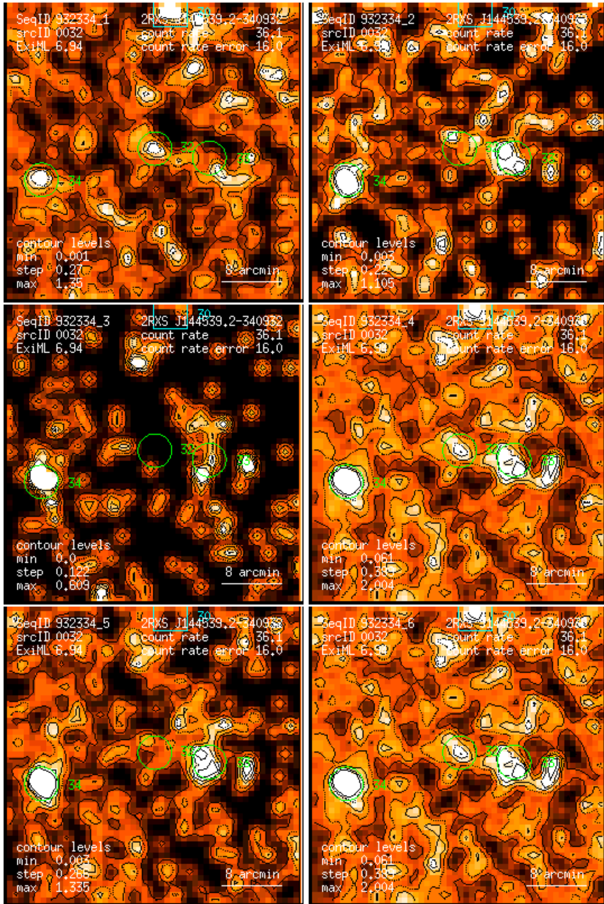
Figure 32: RASS 932334: detection 0032: band rate images, Gaussian filter: (1) PSPC channels 11 – 41, (2) 52 – 90, (3) 91 – 201, (4) 11 – 235, (5) 52 – 201, (6) 11 – 201. Broad band rates in counts/ks. Band rate contour levels in counts/ks/arcmin 2 .
