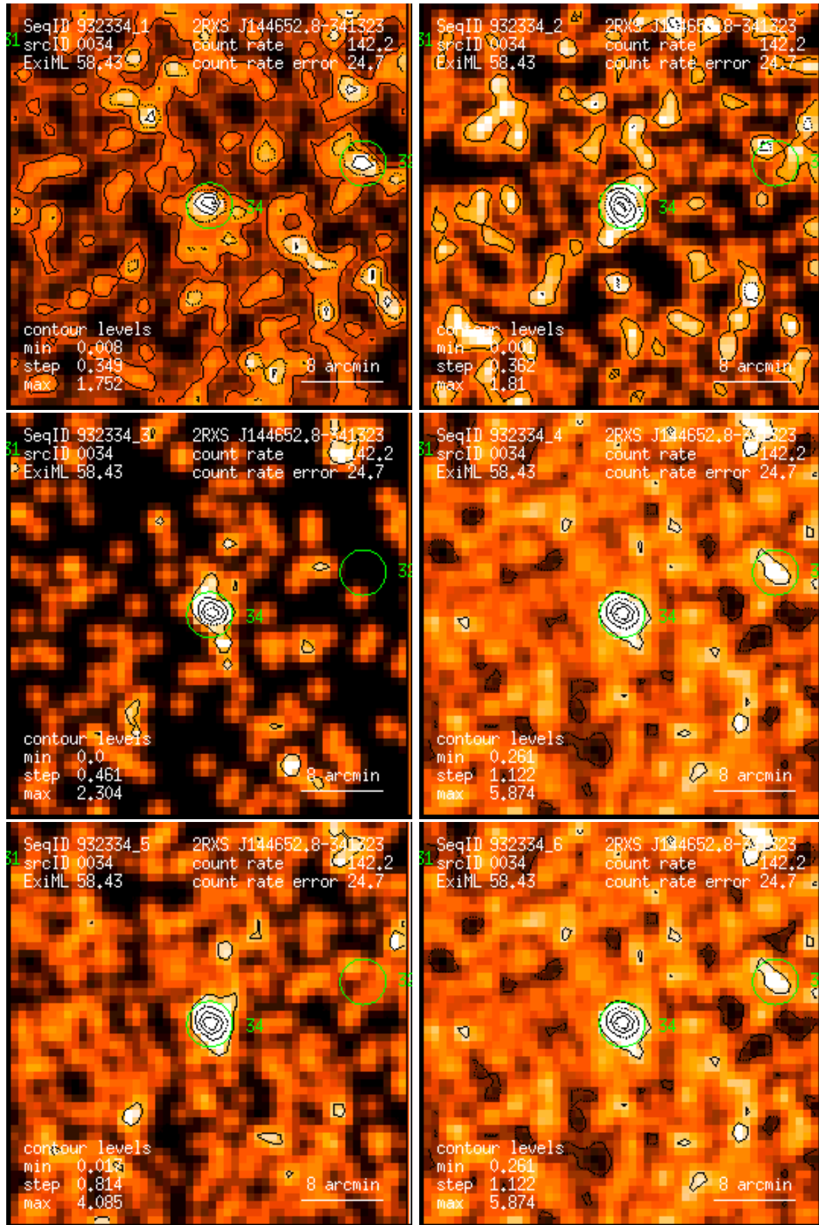
Figure 34: RASS 932334: detection 0034: band rate images, Gaussian filter: (1) PSPC channels 11 – 41, (2) 52 – 90, (3) 91 – 201, (4) 11 – 235, (5) 52 – 201, (6) 11 – 201. Broad band rates in counts/ks. Band rate contour levels in counts/ks/arcmin 2 .
