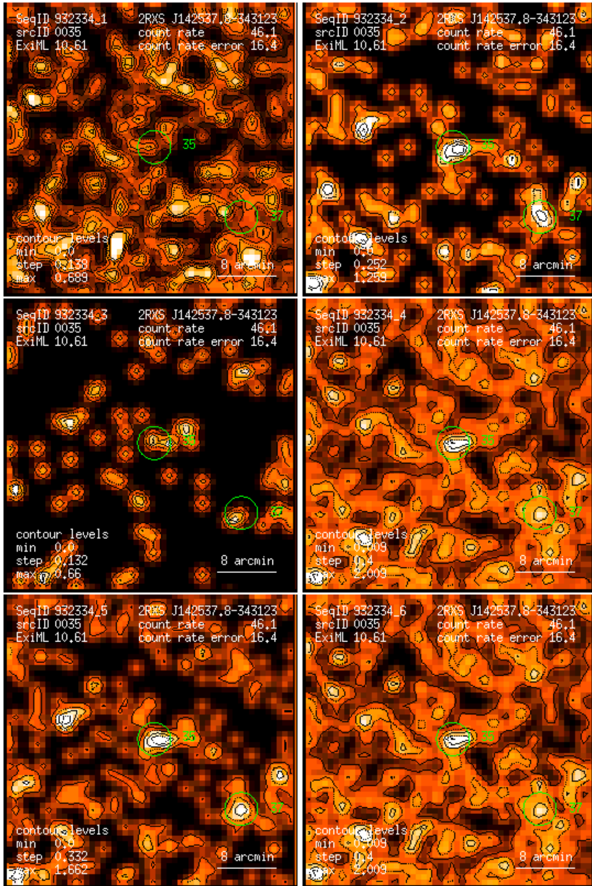
Figure 35: RASS 932334: detection 0035: band rate images, Gaussian filter: (1) PSPC channels 11 – 41, (2) 52 – 90, (3) 91 – 201, (4) 11 – 235, (5) 52 – 201, (6) 11 – 201. Broad band rates in counts/ks. Band rate contour levels in counts/ks/arcmin 2 .
