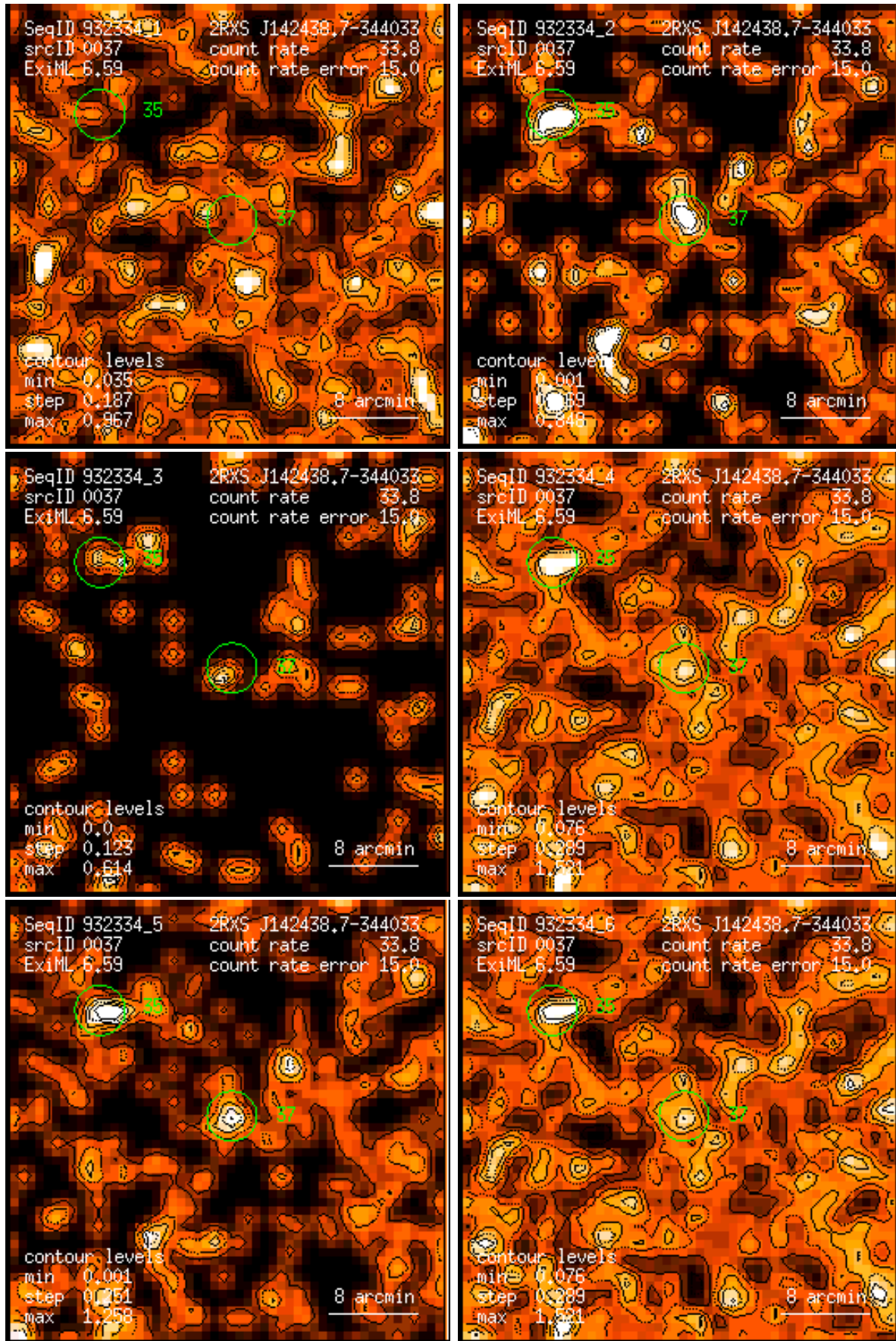
Figure 37: RASS 932334: detection 0037: band rate images, Gaussian filter: (1) PSPC channels 11 – 41, (2) 52 – 90, (3) 91 – 201, (4) 11 – 235, (5) 52 – 201, (6) 11 – 201. Broad band rates in counts/ks. Band rate contour levels in counts/ks/arcmin 2 .
