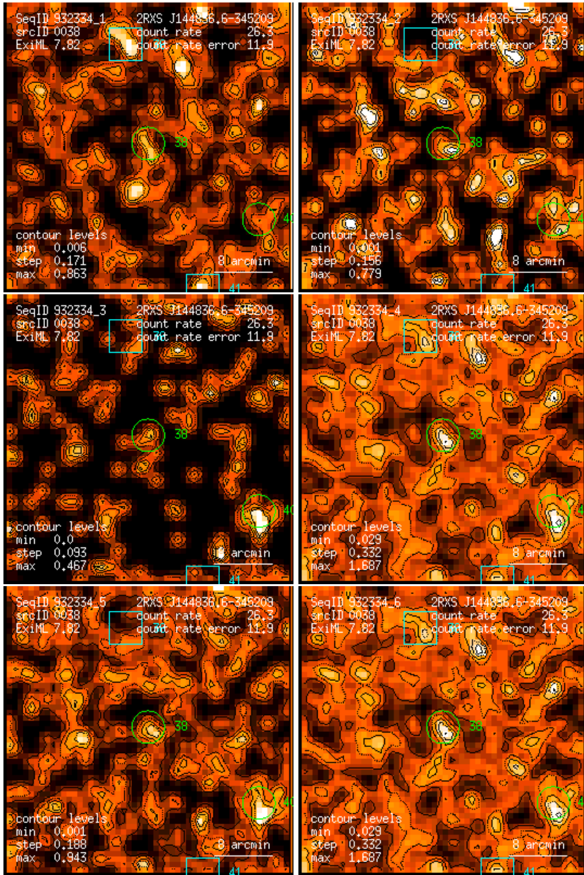
Figure 38: RASS 932334: detection 0038: band rate images, Gaussian filter: (1) PSPC channels 11 – 41, (2) 52 – 90, (3) 91 – 201, (4) 11 – 235, (5) 52 – 201, (6) 11 – 201. Broad band rates in counts/ks. Band rate contour levels in counts/ks/arcmin 2 .
