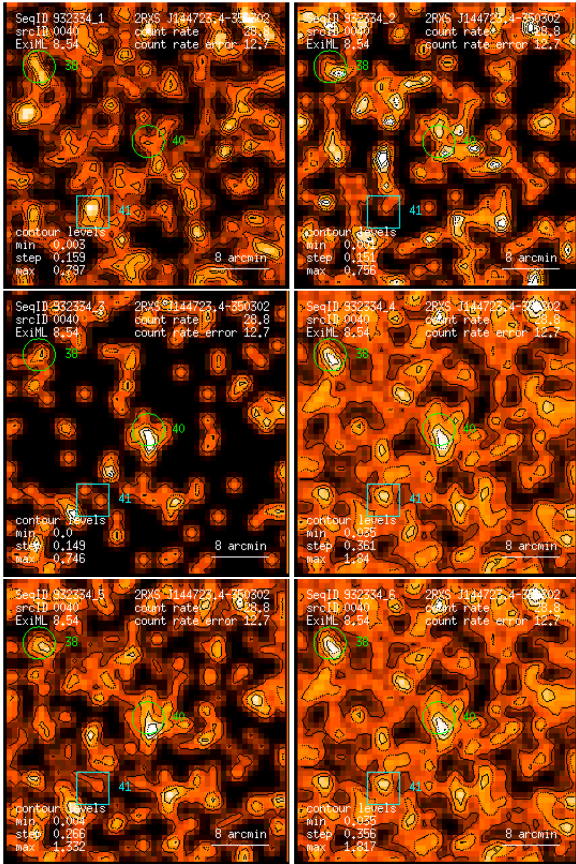
Figure 40: RASS 932334: detection 0040: band rate images, Gaussian filter: (1) PSPC channels 11 – 41, (2) 52 – 90, (3) 91 – 201, (4) 11 – 235, (5) 52 – 201, (6) 11 – 201. Broad band rates in counts/ks. Band rate contour levels in counts/ks/arcmin 2 .
