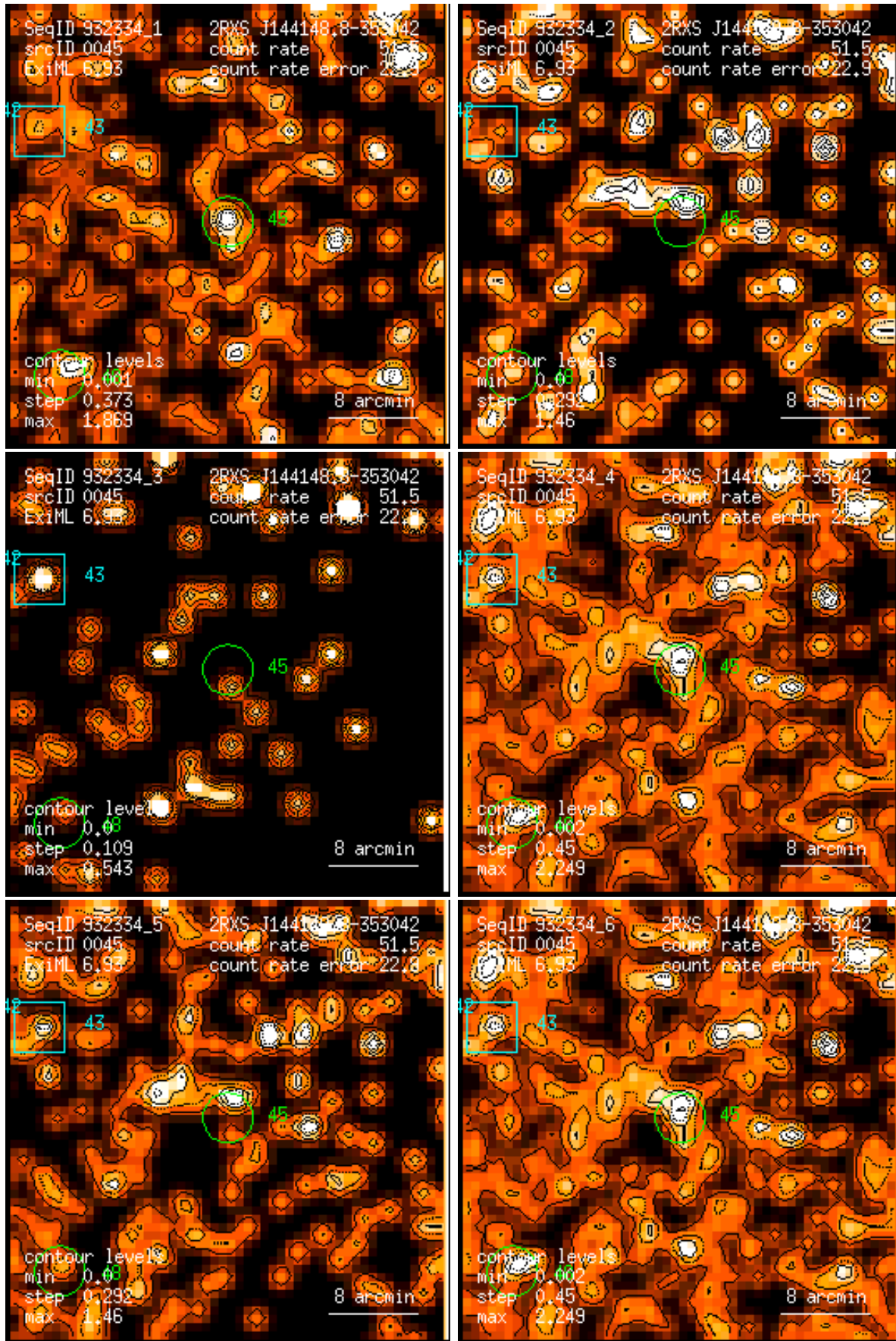
Figure 45: RASS 932334: detection 0045: band rate images, Gaussian filter: (1) PSPC channels 11 – 41, (2) 52 – 90, (3) 91 – 201, (4) 11 – 235, (5) 52 – 201, (6) 11 – 201. Broad band rates in counts/ks. Band rate contour levels in counts/ks/arcmin 2 .
