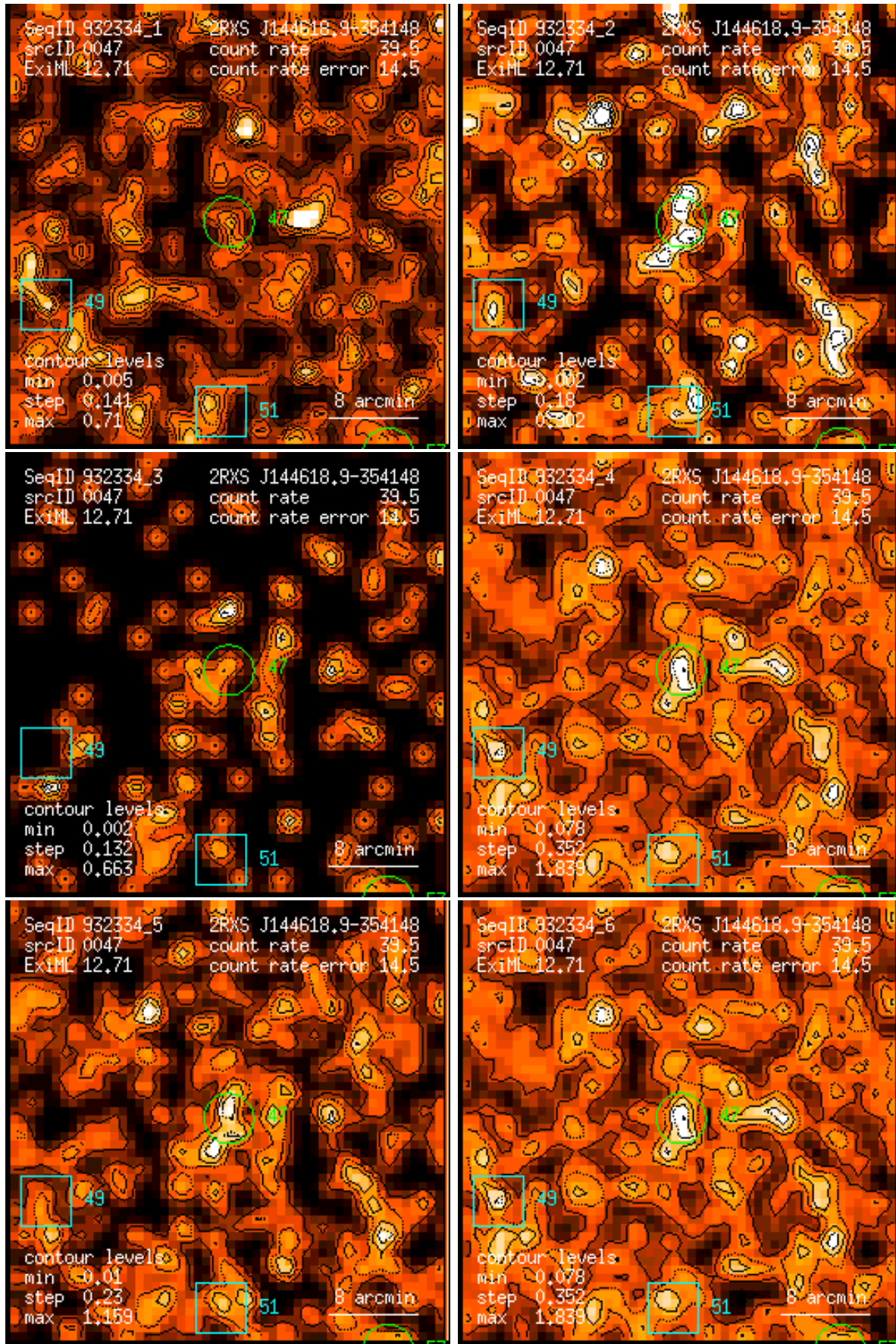
Figure 47: RASS 932334: detection 0047: band rate images, Gaussian filter: (1) PSPC channels 11 – 41, (2) 52 – 90, (3) 91 – 201, (4) 11 – 235, (5) 52 – 201, (6) 11 – 201. Broad band rates in counts/ks. Band rate contour levels in counts/ks/arcmin 2 .
