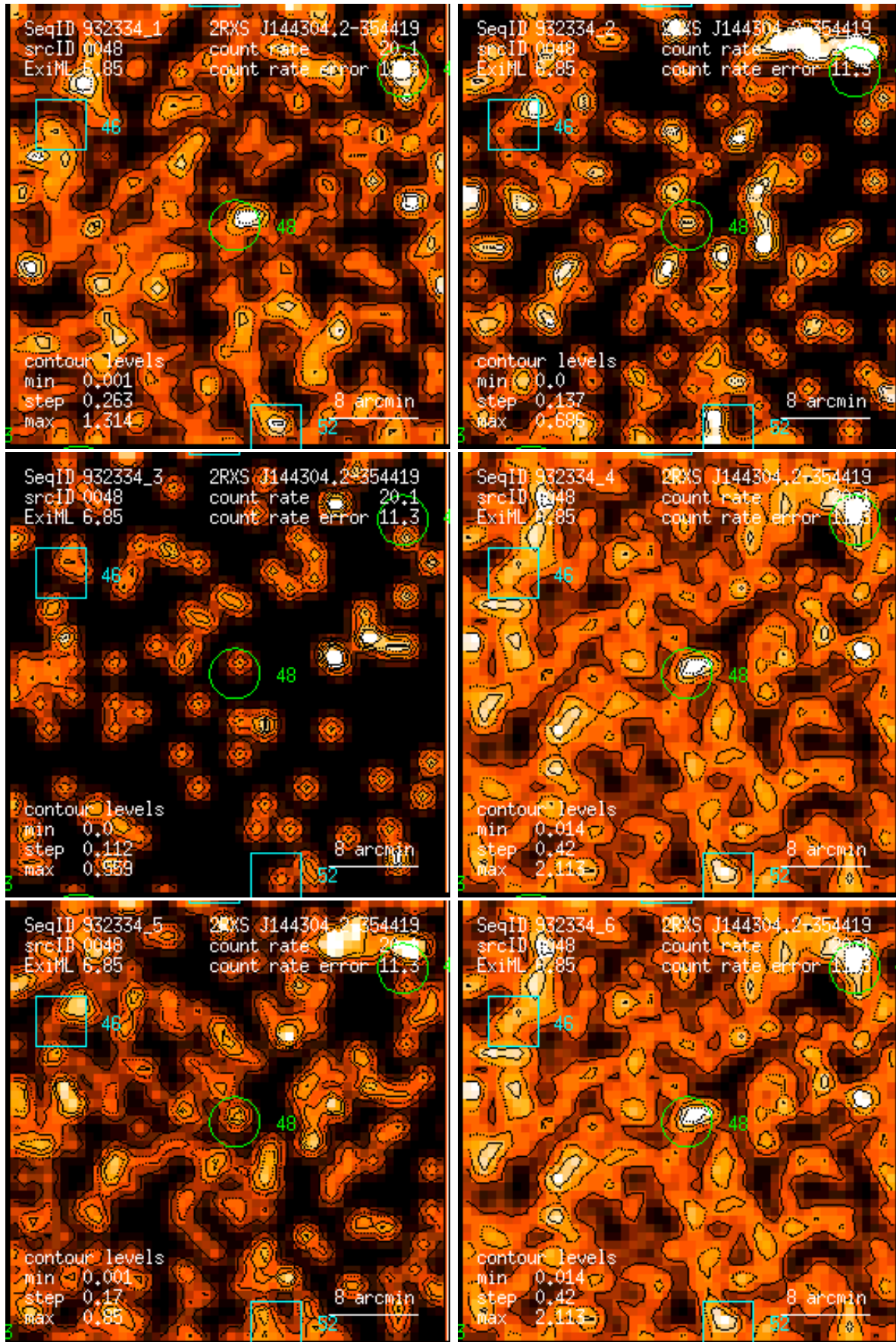
Figure 48: RASS 932334: detection 0048: band rate images, Gaussian filter: (1) PSPC channels 11 – 41, (2) 52 – 90, (3) 91 – 201, (4) 11 – 235, (5) 52 – 201, (6) 11 – 201. Broad band rates in counts/ks. Band rate contour levels in counts/ks/arcmin 2 .
