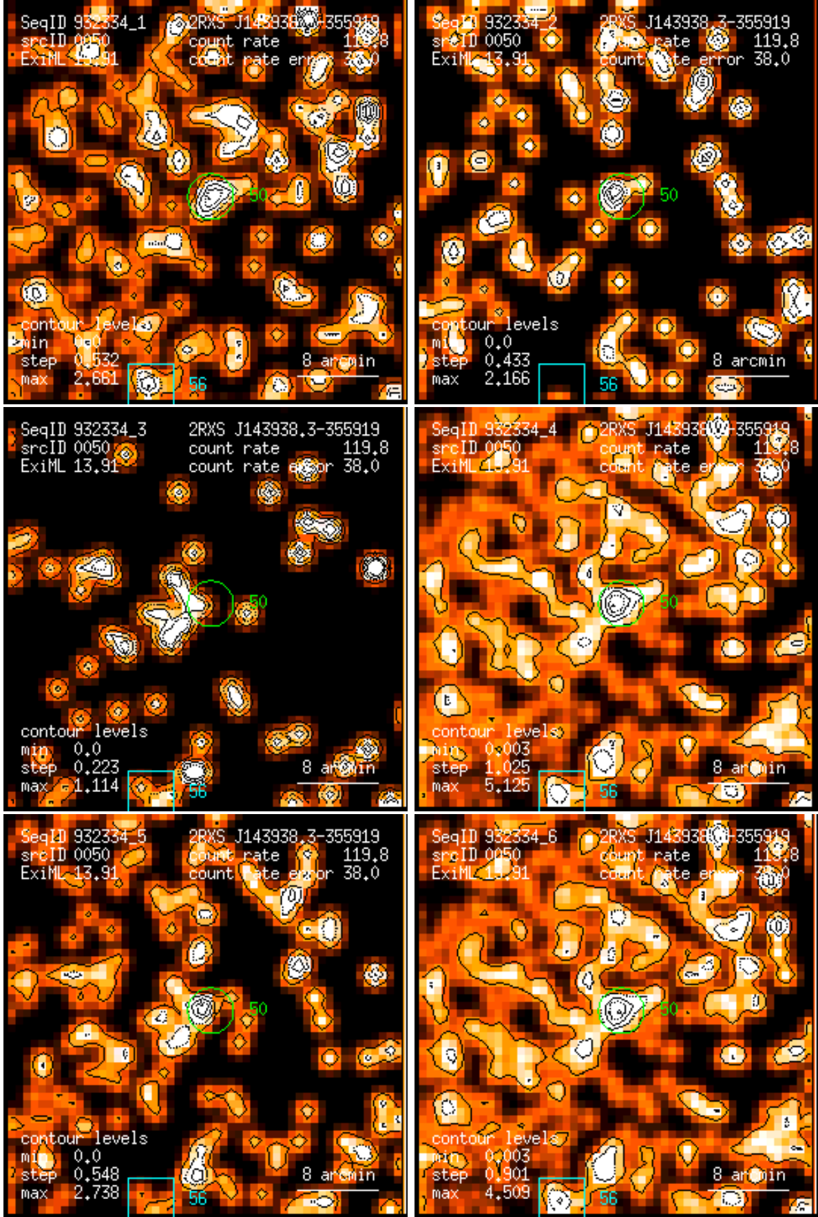
Figure 50: RASS 932334: detection 0050: band rate images, Gaussian filter: (1) PSPC channels 11 – 41, (2) 52 – 90, (3) 91 – 201, (4) 11 – 235, (5) 52 – 201, (6) 11 – 201. Broad band rates in counts/ks. Band rate contour levels in counts/ks/arcmin 2 .
