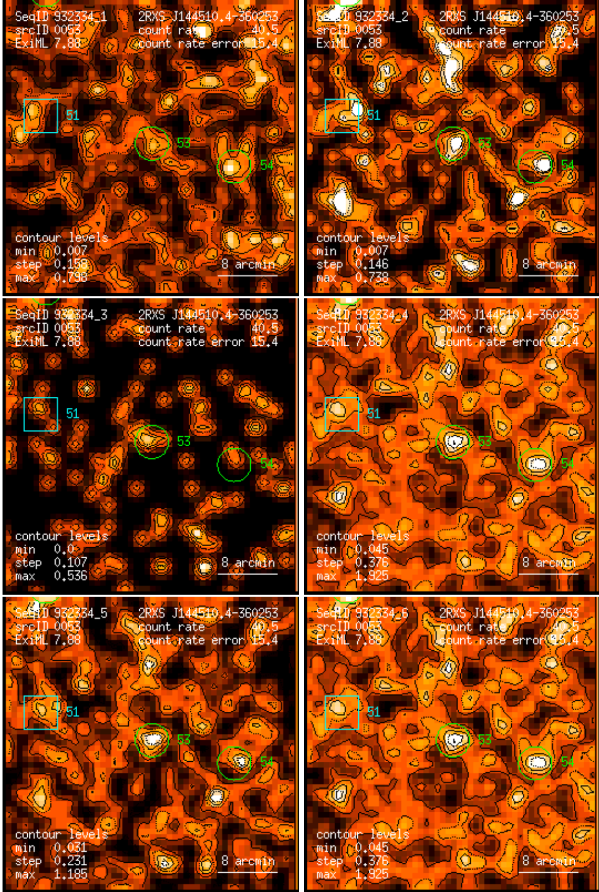
Figure 53: RASS 932334: detection 0053: band rate images, Gaussian filter: (1) PSPC channels 11 – 41, (2) 52 – 90, (3) 91 – 201, (4) 11 – 235, (5) 52 – 201, (6) 11 – 201. Broad band rates in counts/ks. Band rate contour levels in counts/ks/arcmin 2 .
