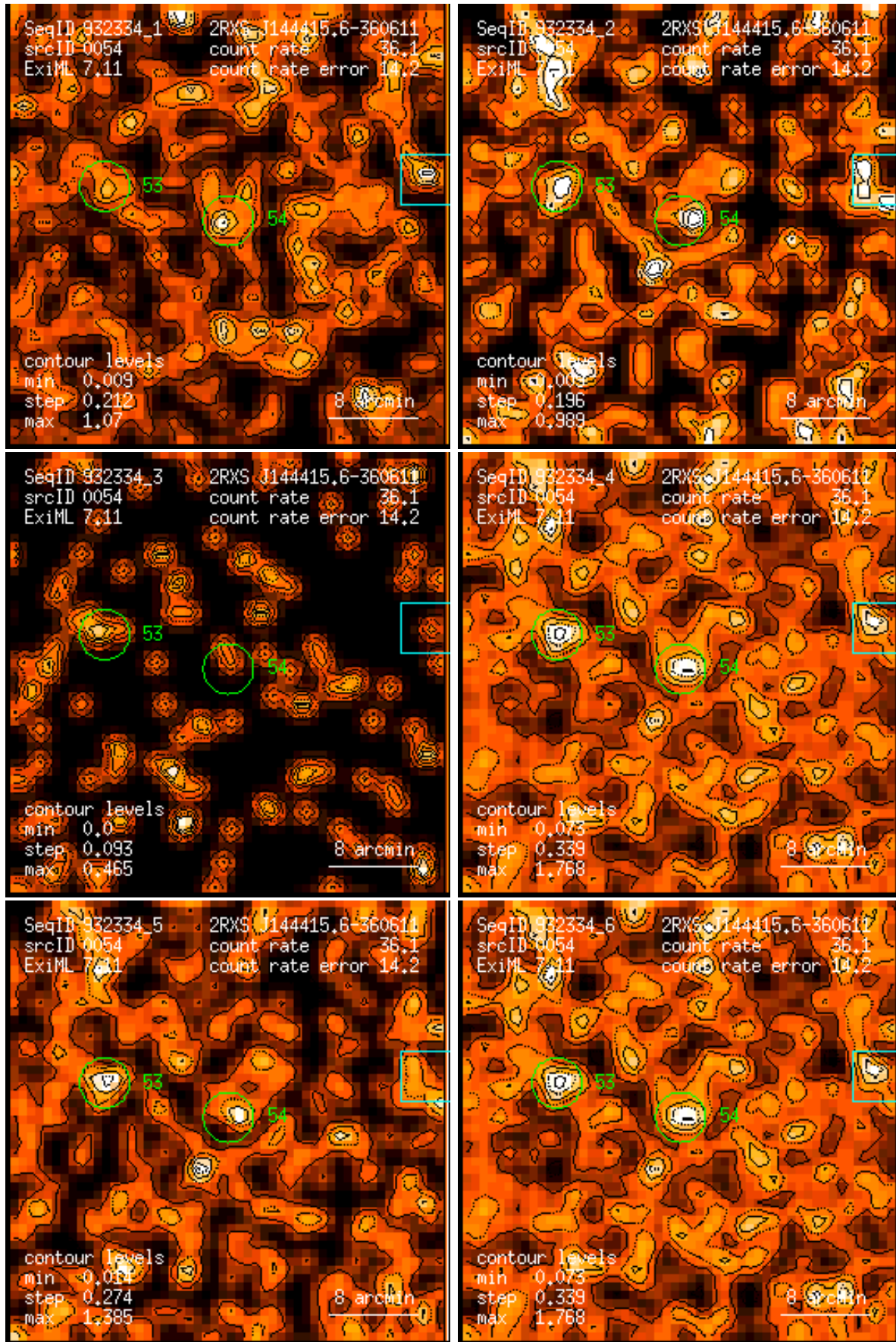
Figure 54: RASS 932334: detection 0054: band rate images, Gaussian filter: (1) PSPC channels 11 – 41, (2) 52 – 90, (3) 91 – 201, (4) 11 – 235, (5) 52 – 201, (6) 11 – 201. Broad band rates in counts/ks. Band rate contour levels in counts/ks/arcmin 2 .
