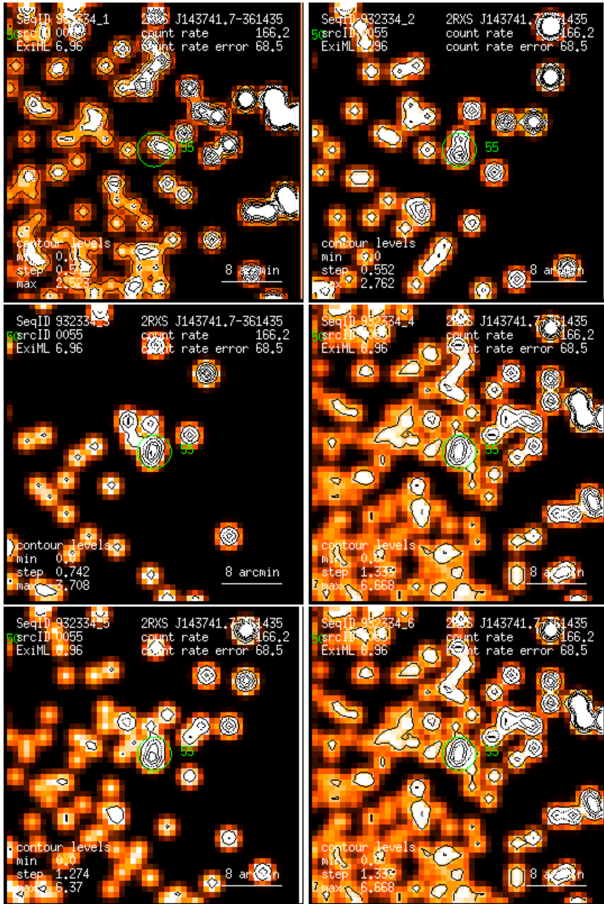
Figure 55: RASS 932334: detection 0055: band rate images, Gaussian filter: (1) PSPC channels 11 – 41, (2) 52 – 90, (3) 91 – 201, (4) 11 – 235, (5) 52 – 201, (6) 11 – 201. Broad band rates in counts/ks. Band rate contour levels in counts/ks/arcmin 2 .
