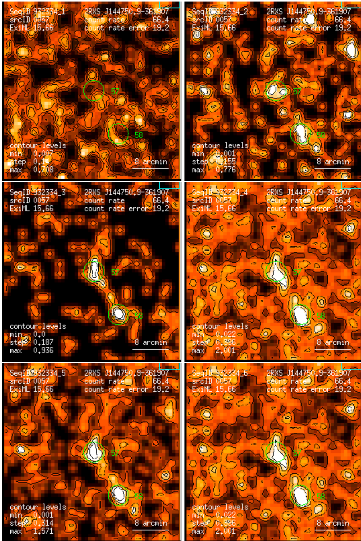
Figure 57: RASS 932334: detection 0057: band rate images, Gaussian filter: (1) PSPC channels 11 – 41, (2) 52 – 90, (3) 91 – 201, (4) 11 – 235, (5) 52 – 201, (6) 11 – 201. Broad band rates in counts/ks. Band rate contour levels in counts/ks/arcmin 2 .
