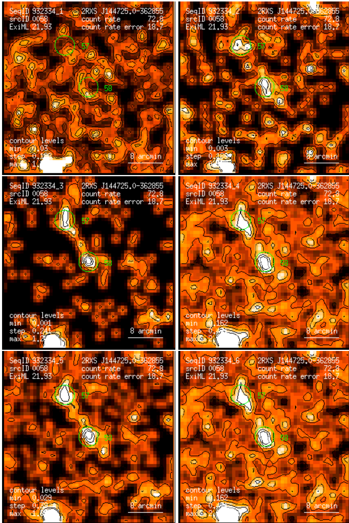
Figure 58: RASS 932334: detection 0058: band rate images, Gaussian filter: (1) PSPC channels 11 – 41, (2) 52 – 90, (3) 91 – 201, (4) 11 – 235, (5) 52 – 201, (6) 11 – 201. Broad band rates in counts/ks. Band rate contour levels in counts/ks/arcmin 2 .
