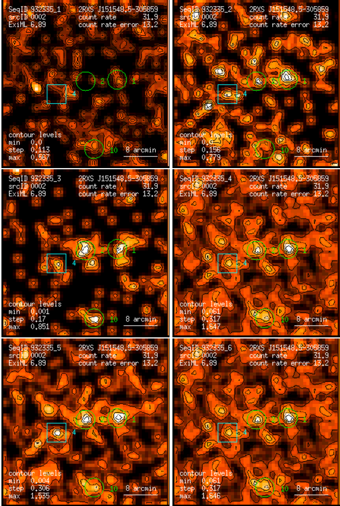
Figure 2: RASS 932335: detection 0002: band rate images, Gaussian filter: (1) PSPC channels 11 – 41, (2) 52 – 90, (3) 91 – 201, (4) 11 – 235, (5) 52 – 201, (6) 11 – 201. Broad band rates in counts/ks. Band rate contour levels in counts/ks/arcmin 2 .
