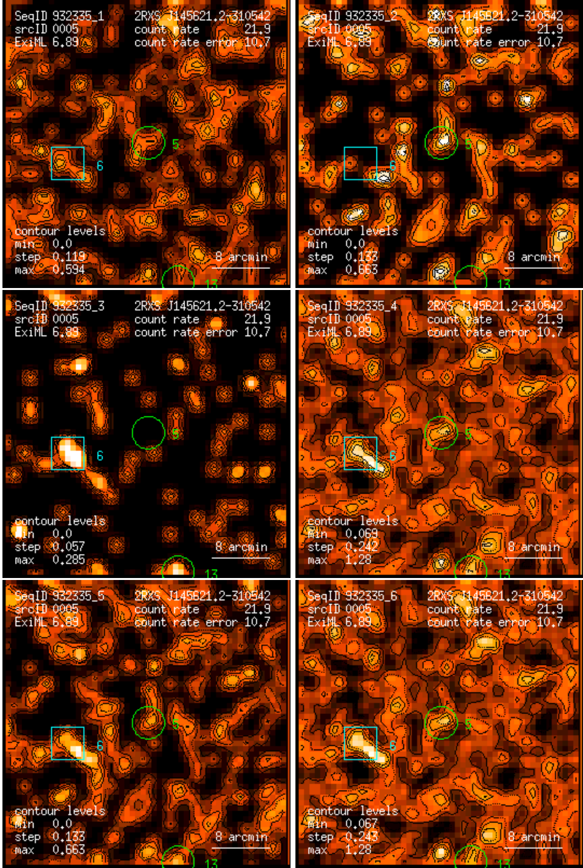
Figure 5: RASS 932335: detection 0005: band rate images, Gaussian filter: (1) PSPC channels 11 – 41, (2) 52 – 90, (3) 91 – 201, (4) 11 – 235, (5) 52 – 201, (6) 11 – 201. Broad band rates in counts/ks. Band rate contour levels in counts/ks/arcmin 2 .
