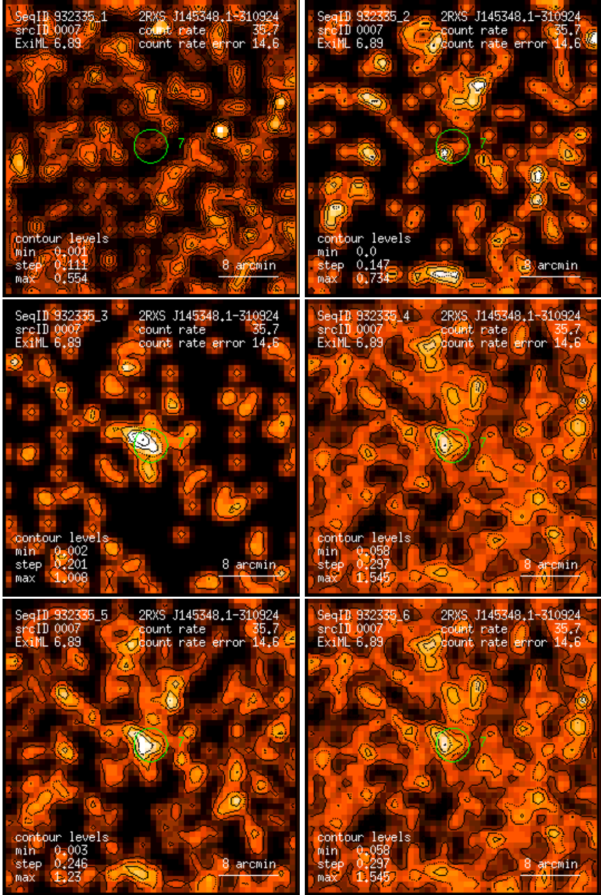
Figure 7: RASS 932335: detection 0007: band rate images, Gaussian filter: (1) PSPC channels 11 – 41, (2) 52 – 90, (3) 91 – 201, (4) 11 – 235, (5) 52 – 201, (6) 11 – 201. Broad band rates in counts/ks. Band rate contour levels in counts/ks/arcmin 2 .
