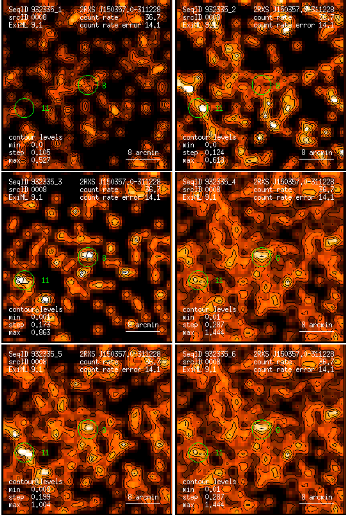
Figure 8: RASS 932335: detection 0008: band rate images, Gaussian filter: (1) PSPC channels 11 – 41, (2) 52 – 90, (3) 91 – 201, (4) 11 – 235, (5) 52 – 201, (6) 11 – 201. Broad band rates in counts/ks. Band rate contour levels in counts/ks/arcmin 2 .
