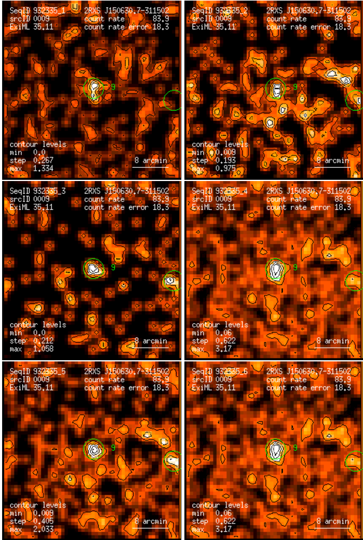
Figure 9: RASS 932335: detection 0009: band rate images, Gaussian filter: (1) PSPC channels 11 – 41, (2) 52 – 90, (3) 91 – 201, (4) 11 – 235, (5) 52 – 201, (6) 11 – 201. Broad band rates in counts/ks. Band rate contour levels in counts/ks/arcmin 2 .
