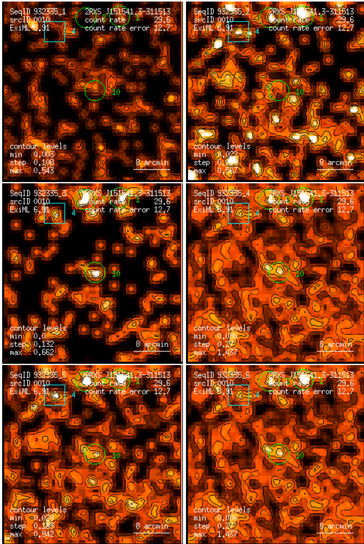
Figure 10: RASS 932335: detection 0010: band rate images, Gaussian filter: (1) PSPC channels 11 – 41, (2) 52 – 90, (3) 91 – 201, (4) 11 – 235, (5) 52 – 201, (6) 11 – 201. Broad band rates in counts/ks. Band rate contour levels in counts/ks/arcmin 2 .
