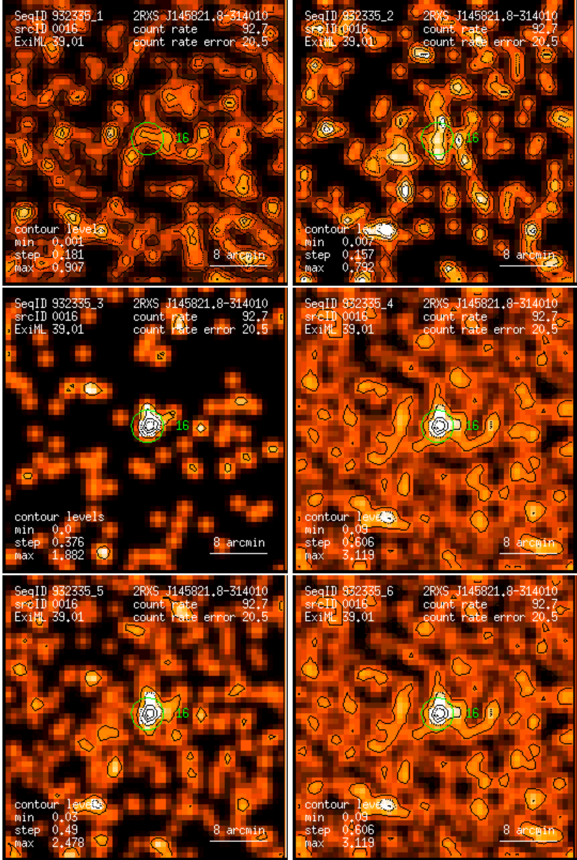
Figure 16: RASS 932335: detection 0016: band rate images, Gaussian filter: (1) PSPC channels 11 – 41, (2) 52 – 90, (3) 91 – 201, (4) 11 – 235, (5) 52 – 201, (6) 11 – 201. Broad band rates in counts/ks. Band rate contour levels in counts/ks/arcmin 2 .
