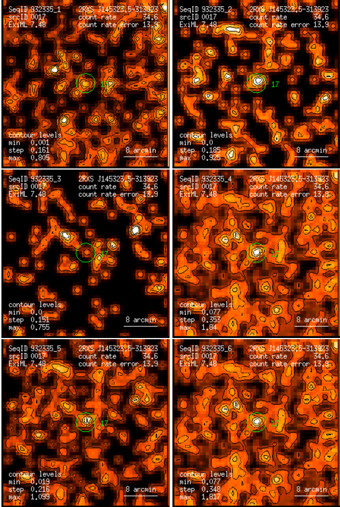
Figure 17: RASS 932335: detection 0017: band rate images, Gaussian filter: (1) PSPC channels 11 – 41, (2) 52 – 90, (3) 91 – 201, (4) 11 – 235, (5) 52 – 201, (6) 11 – 201. Broad band rates in counts/ks. Band rate contour levels in counts/ks/arcmin 2 .
