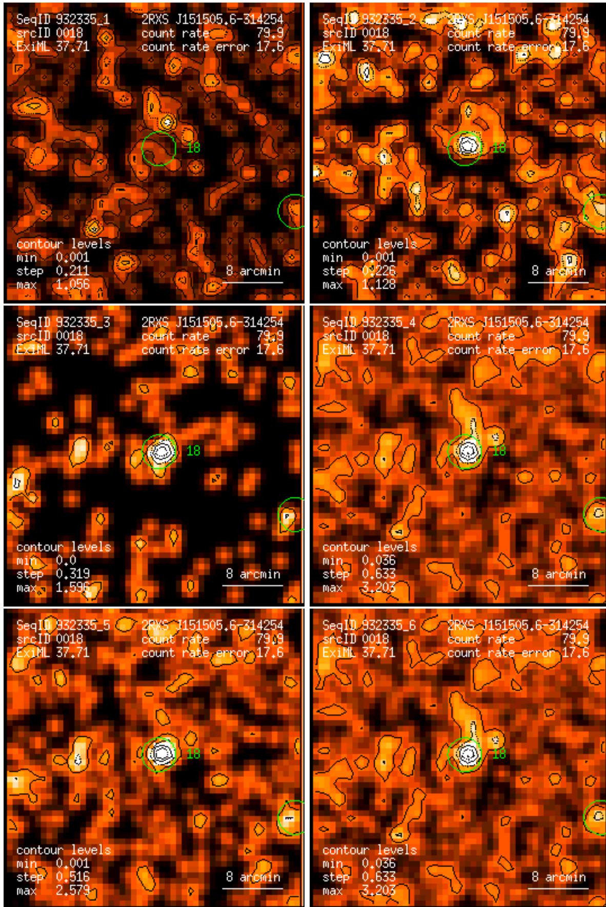
Figure 18: RASS 932335: detection 0018: band rate images, Gaussian filter: (1) PSPC channels 11 – 41, (2) 52 – 90, (3) 91 – 201, (4) 11 – 235, (5) 52 – 201, (6) 11 – 201. Broad band rates in counts/ks. Band rate contour levels in counts/ks/arcmin 2 .
