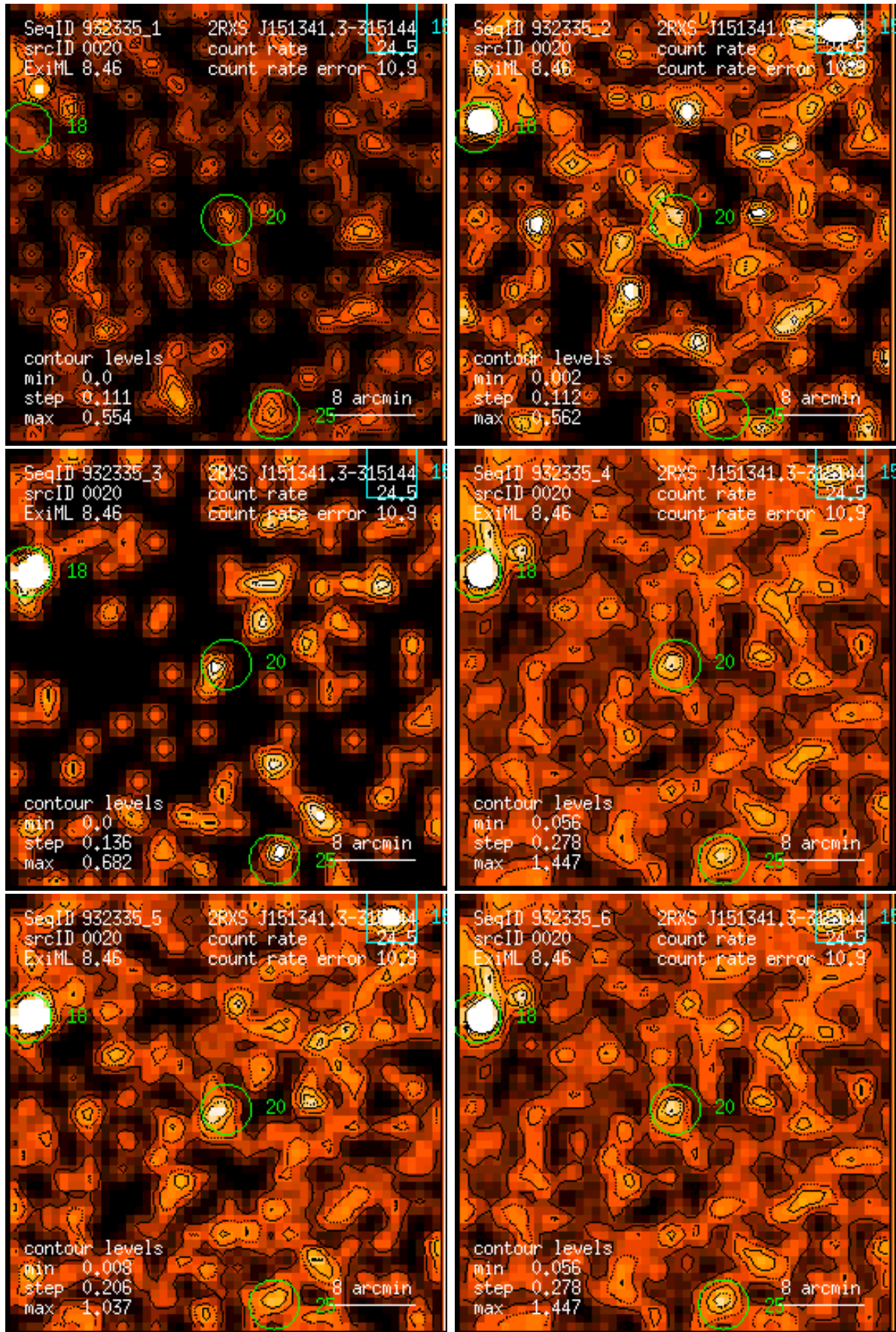
Figure 20: RASS 932335: detection 0020: band rate images, Gaussian filter: (1) PSPC channels 11 – 41, (2) 52 – 90, (3) 91 – 201, (4) 11 – 235, (5) 52 – 201, (6) 11 – 201. Broad band rates in counts/ks. Band rate contour levels in counts/ks/arcmin 2 .
