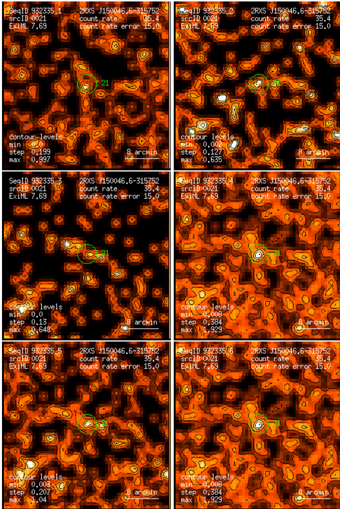
Figure 21: RASS 932335: detection 0021: band rate images, Gaussian filter: (1) PSPC channels 11 – 41, (2) 52 – 90, (3) 91 – 201, (4) 11 – 235, (5) 52 – 201, (6) 11 – 201. Broad band rates in counts/ks. Band rate contour levels in counts/ks/arcmin 2 .
