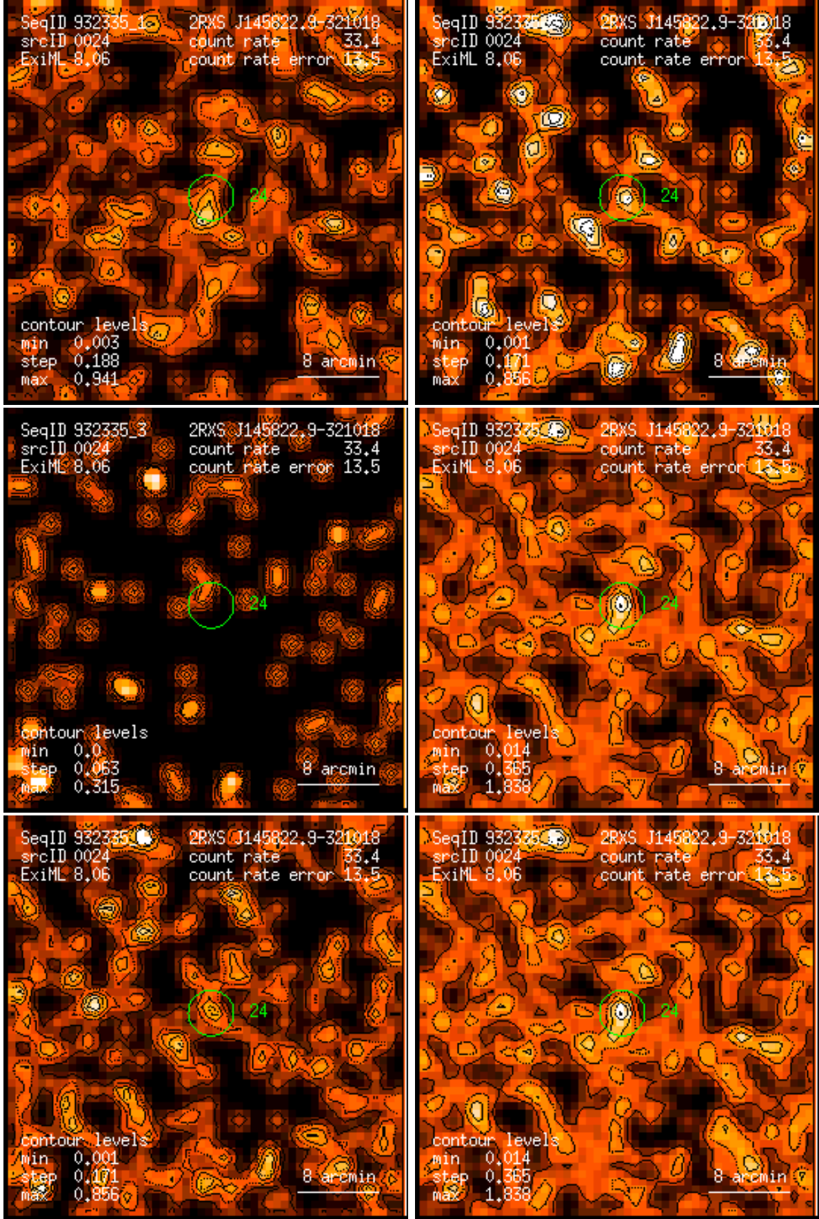
Figure 24: RASS 932335: detection 0024: band rate images, Gaussian filter: (1) PSPC channels 11 – 41, (2) 52 – 90, (3) 91 – 201, (4) 11 – 235, (5) 52 – 201, (6) 11 – 201. Broad band rates in counts/ks. Band rate contour levels in counts/ks/arcmin 2 .
