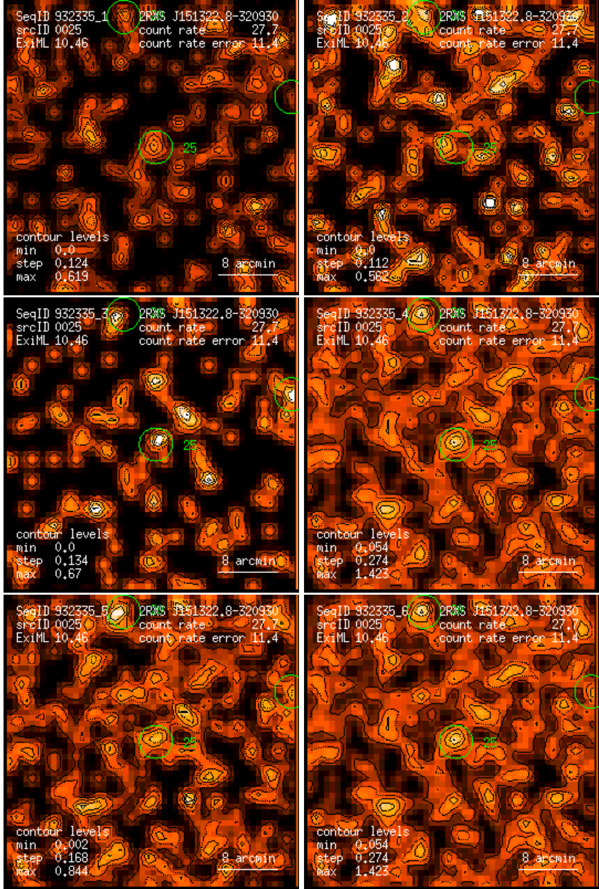
Figure 25: RASS 932335: detection 0025: band rate images, Gaussian filter: (1) PSPC channels 11 – 41, (2) 52 – 90, (3) 91 – 201, (4) 11 – 235, (5) 52 – 201, (6) 11 – 201. Broad band rates in counts/ks. Band rate contour levels in counts/ks/arcmin 2 .
