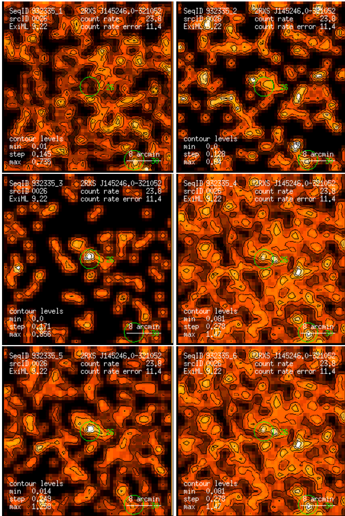
Figure 26: RASS 932335: detection 0026: band rate images, Gaussian filter: (1) PSPC channels 11 – 41, (2) 52 – 90, (3) 91 – 201, (4) 11 – 235, (5) 52 – 201, (6) 11 – 201. Broad band rates in counts/ks. Band rate contour levels in counts/ks/arcmin 2 .
