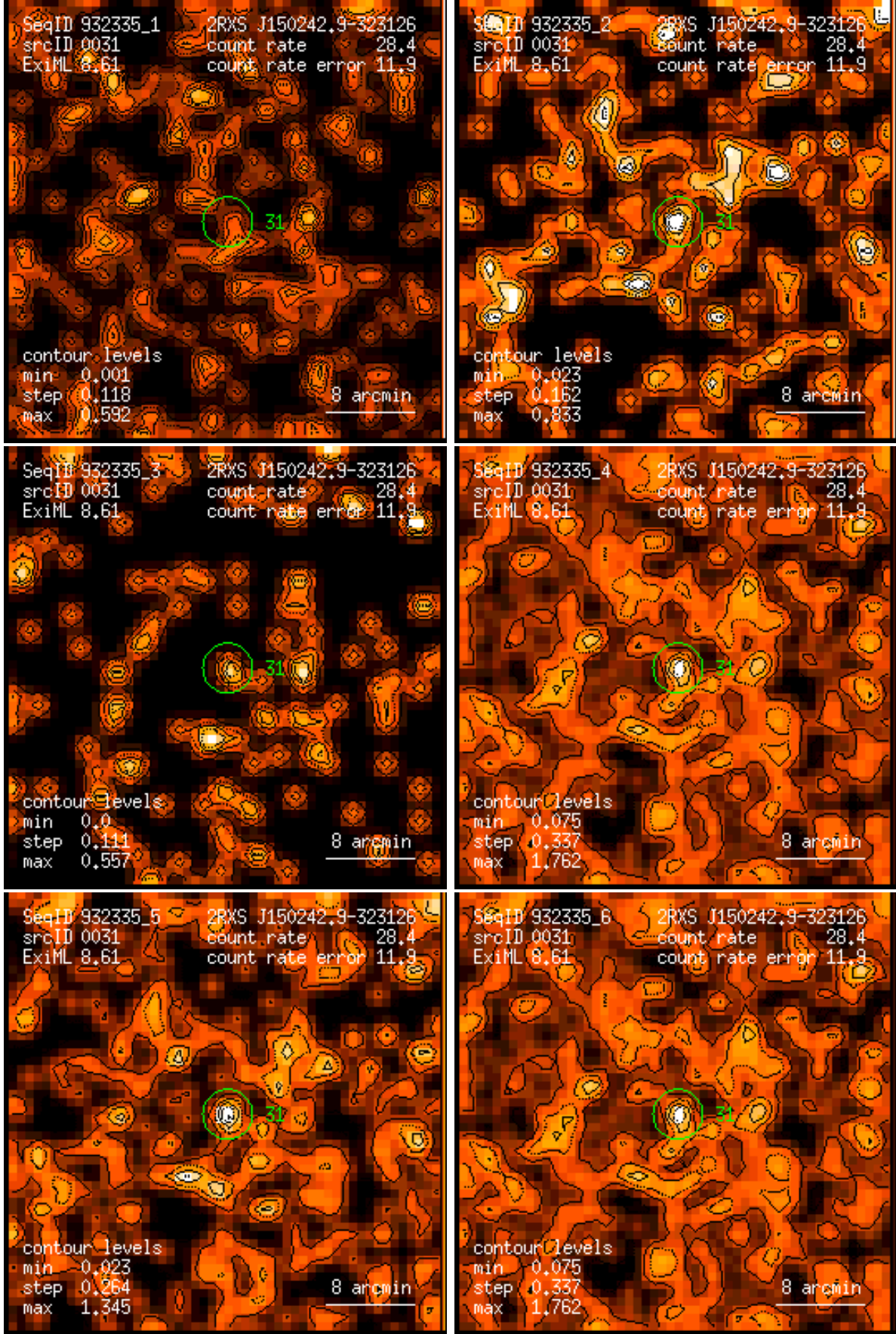
Figure 31: RASS 932335: detection 0031: band rate images, Gaussian filter: (1) PSPC channels 11 – 41, (2) 52 – 90, (3) 91 – 201, (4) 11 – 235, (5) 52 – 201, (6) 11 – 201. Broad band rates in counts/ks. Band rate contour levels in counts/ks/arcmin 2 .
