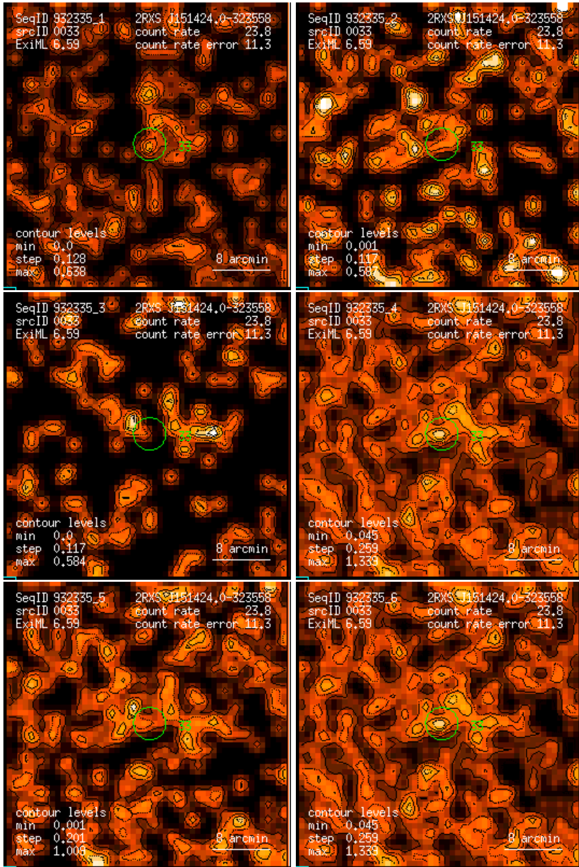
Figure 33: RASS 932335: detection 0033: band rate images, Gaussian filter: (1) PSPC channels 11 – 41, (2) 52 – 90, (3) 91 – 201, (4) 11 – 235, (5) 52 – 201, (6) 11 – 201. Broad band rates in counts/ks. Band rate contour levels in counts/ks/arcmin 2 .
