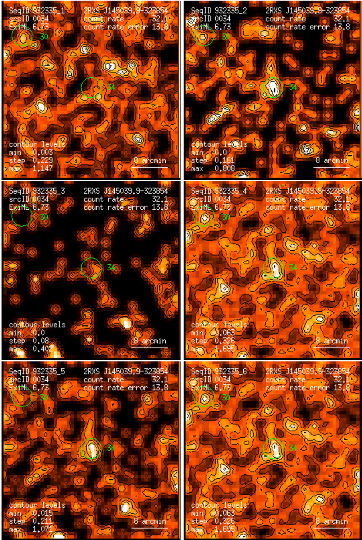
Figure 34: RASS 932335: detection 0034: band rate images, Gaussian filter: (1) PSPC channels 11 – 41, (2) 52 – 90, (3) 91 – 201, (4) 11 – 235, (5) 52 – 201, (6) 11 – 201. Broad band rates in counts/ks. Band rate contour levels in counts/ks/arcmin 2 .
