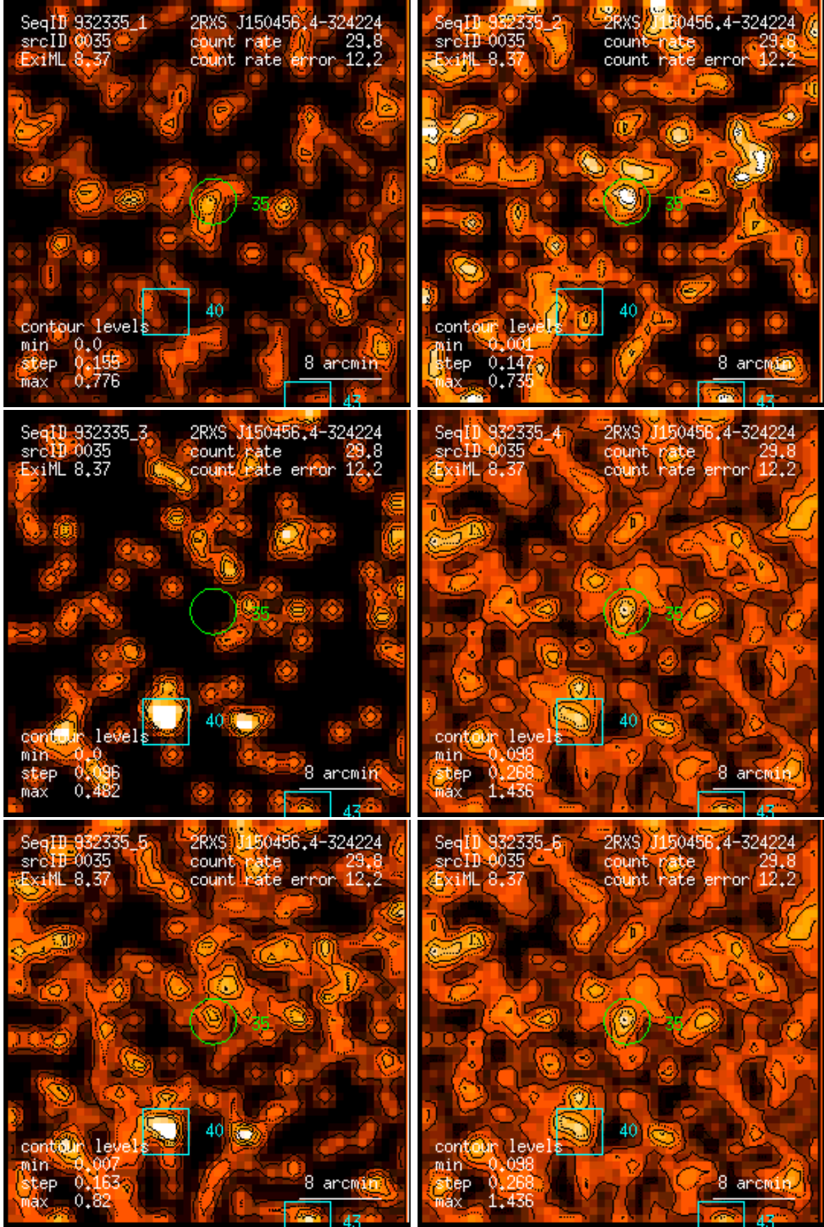
Figure 35: RASS 932335: detection 0035: band rate images, Gaussian filter: (1) PSPC channels 11 – 41, (2) 52 – 90, (3) 91 – 201, (4) 11 – 235, (5) 52 – 201, (6) 11 – 201. Broad band rates in counts/ks. Band rate contour levels in counts/ks/arcmin 2 .
