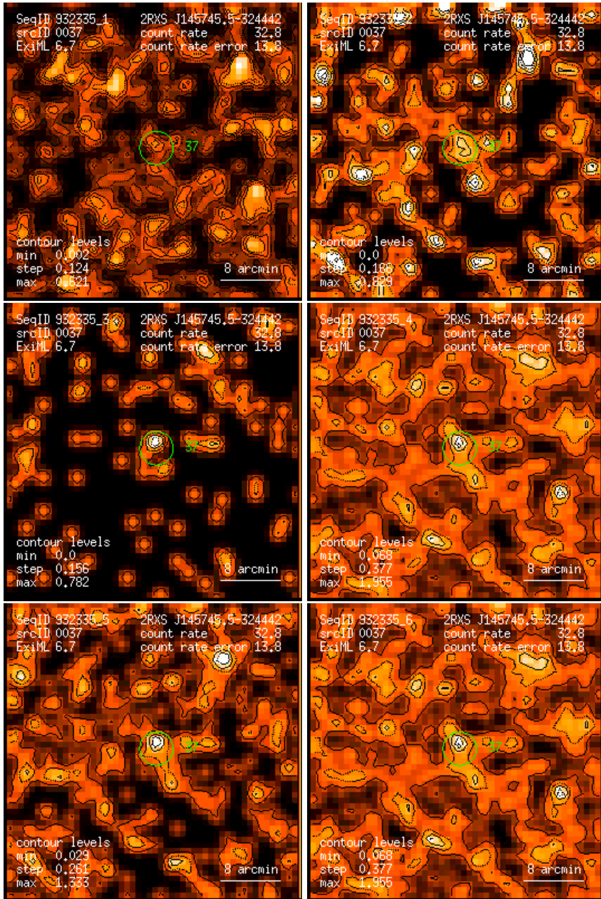
Figure 37: RASS 932335: detection 0037: band rate images, Gaussian filter: (1) PSPC channels 11 – 41, (2) 52 – 90, (3) 91 – 201, (4) 11 – 235, (5) 52 – 201, (6) 11 – 201. Broad band rates in counts/ks. Band rate contour levels in counts/ks/arcmin 2 .
