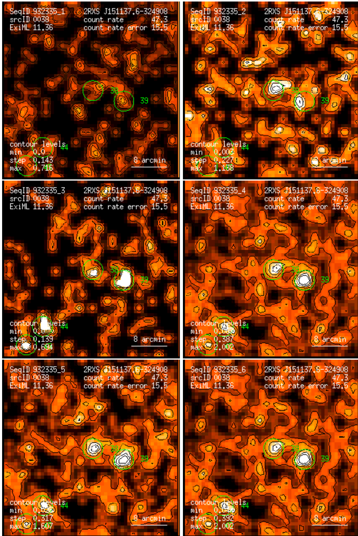
Figure 38: RASS 932335: detection 0038: band rate images, Gaussian filter: (1) PSPC channels 11 – 41, (2) 52 – 90, (3) 91 – 201, (4) 11 – 235, (5) 52 – 201, (6) 11 – 201. Broad band rates in counts/ks. Band rate contour levels in counts/ks/arcmin 2 .
